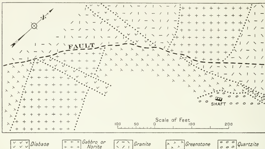
Fig. 28—Plan of ninth level, No. 2 mine, Canadian Copper Company, Copper Cliff, Ontario, showing fault. The dike has been faulted 350 feet to the southwest, but the vertical displacement is not known. From plans of the Canadian Copper Company.
